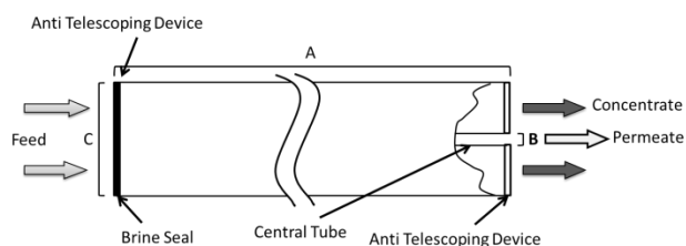
Figure 1: Element Dimensions Diagram - AG8040F-400 LF, ** WET
